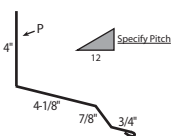
20a GAMBREL FLASHING PF11 4:12 PITCH STANDARD UNLESS SPECIFIED OTHERWISE
