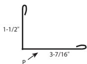
19b NOTCHED TRANSITION FLASHING (41") PF49 4:12 PITCH STANDARD UNLESS SPECIFIED OTHERWISE
