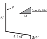
20b NOTCHED GAMBREL FLASHING (41") PF50 4:12 PITCH STANDARD UNLESS SPECIFIED OTHERWISE
