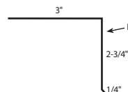
23a 3 x 3 EAVE EDGE FT04 4:12 PITCH STANDARD UNLESS SPECIFIED OTHERWISE
