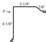
16a END WALL PF08 4:12 PITCH STANDARD UNLESS SPECIFIED OTHERWISE
